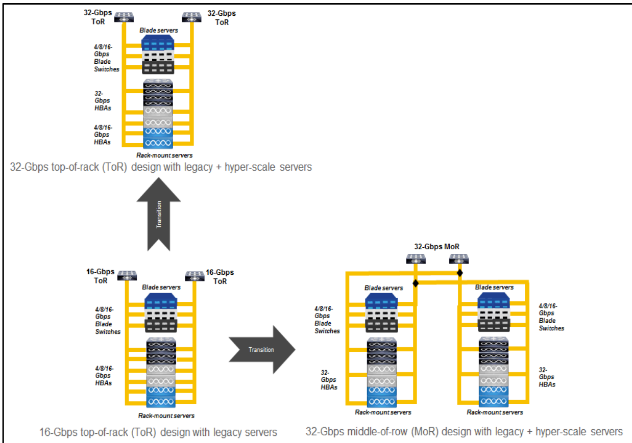
Figure 3. IBM Storage Networking SAN32C-6 in Hyper-scale server environments
