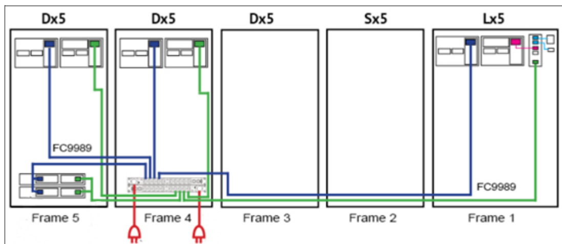
Figure 1-52 Power configuration with Feature Code 1951/1952 (rear view of the library)
