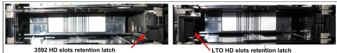
Figure 1-11 HD slot
