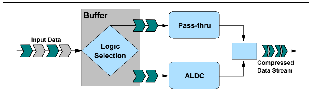
Figure 2-12 LTO-DC block diagram
