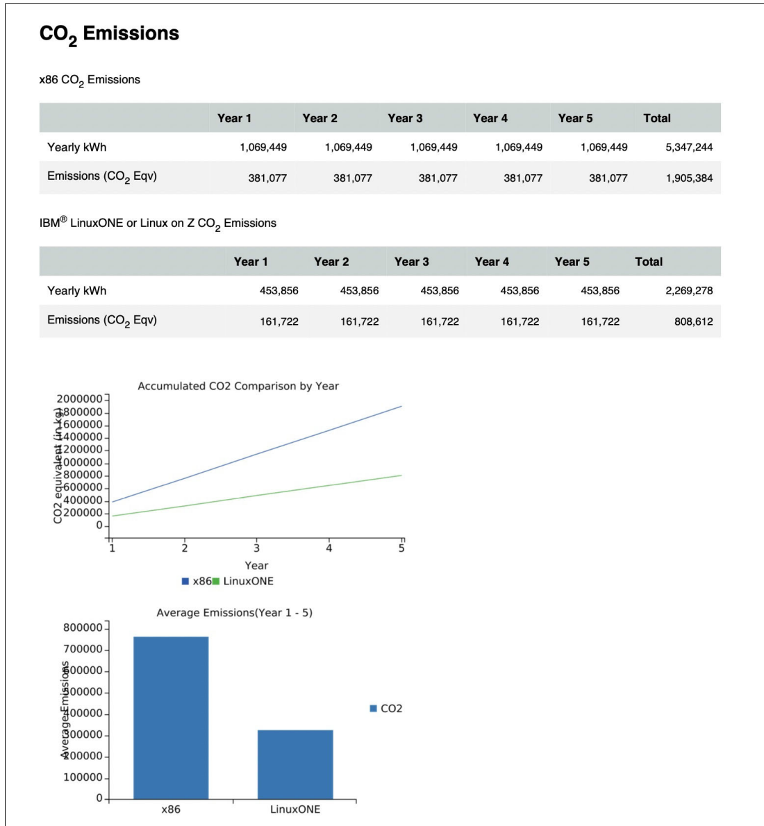
Figure 1-4 Co2 emissions Comparison
