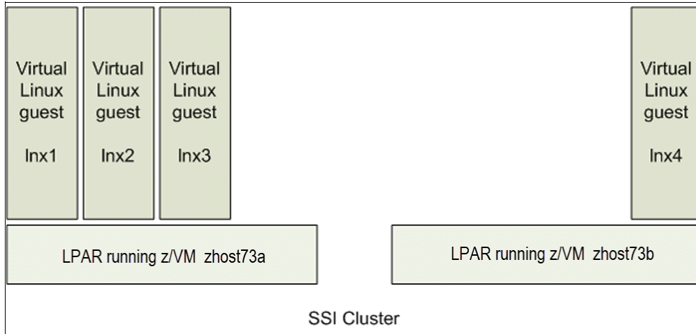
Figure 3-6 Simple representation of SSI cluster before live guest relocation
