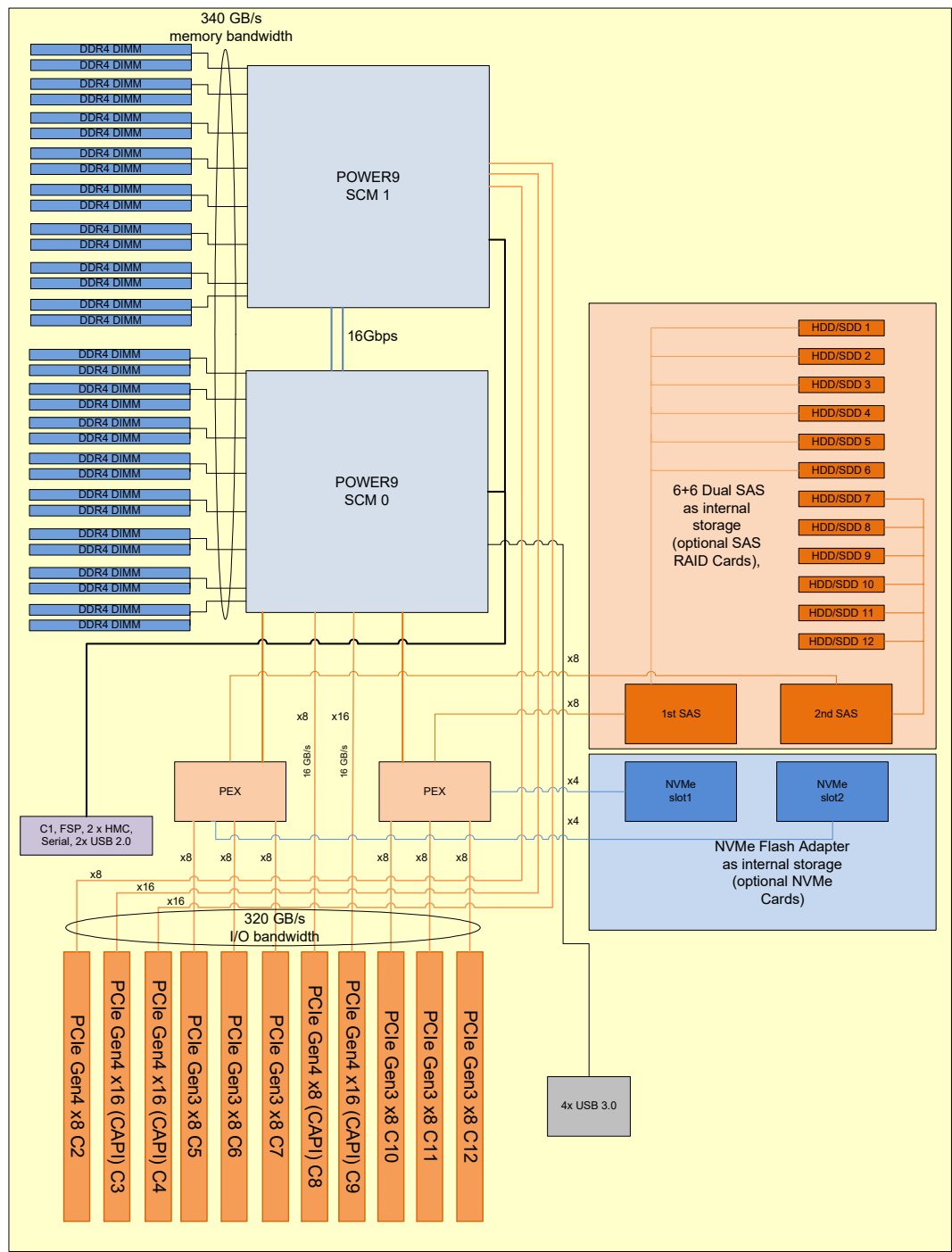
Figure 2-1 The IBM Power H924 logical system diagram
