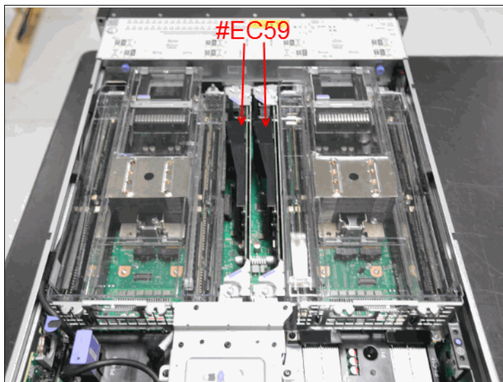
Figure 2-12 Two #EC59 components in a Power H922 server
