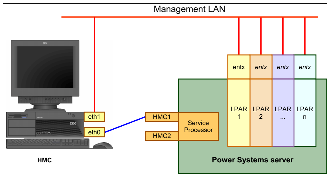
Figure 1-17 Network connections from the HMC to service processor and LPARs
