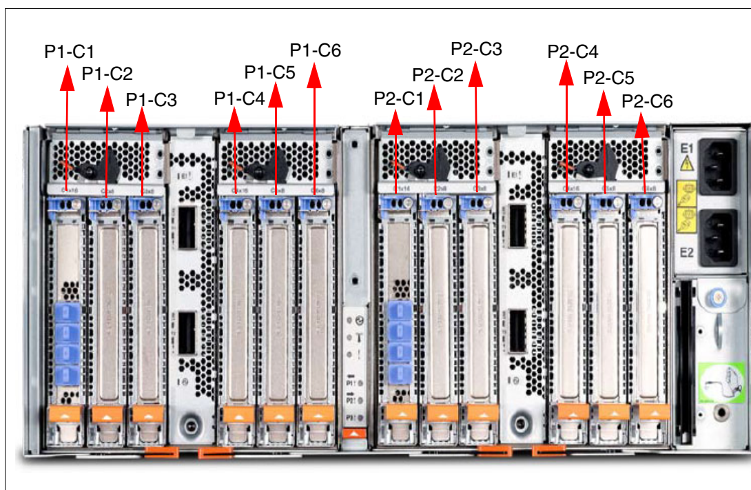
Figure 1-8 Rear view of a PCIe Gen3 I/O expansion drawer with PCIe slots location codes
