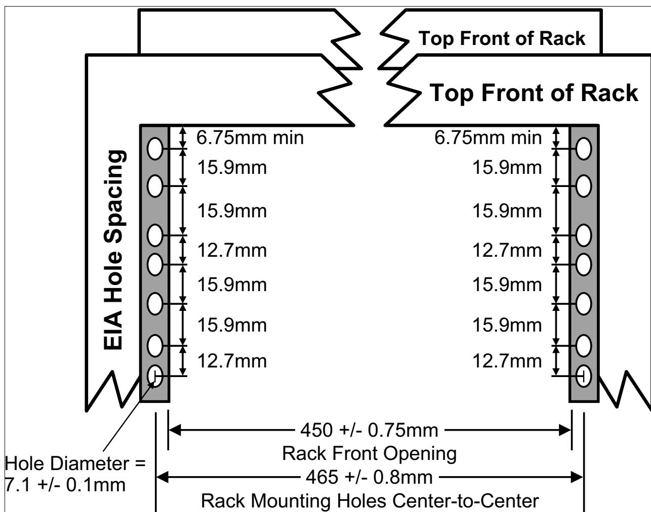
Figure 1-15 Rack specification dimensions: Top front view
