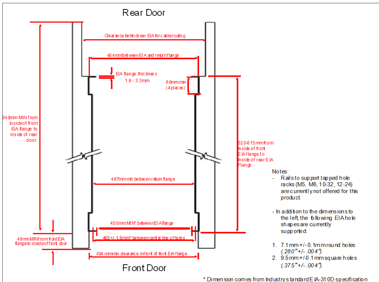
Figure 1-14 Top view of the rack specification dimensions (not specific to IBM)
