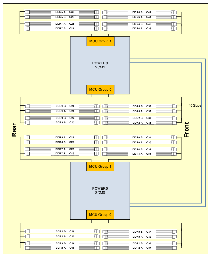
Figure 2-7 Memory DIMM topology for Power H922 and Power H924 servers
