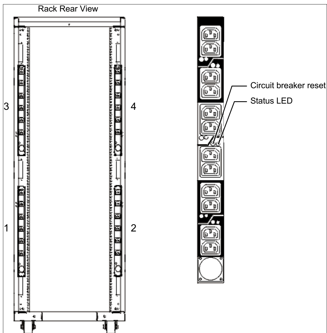
Figure 1-12 PDU placement and PDU view
