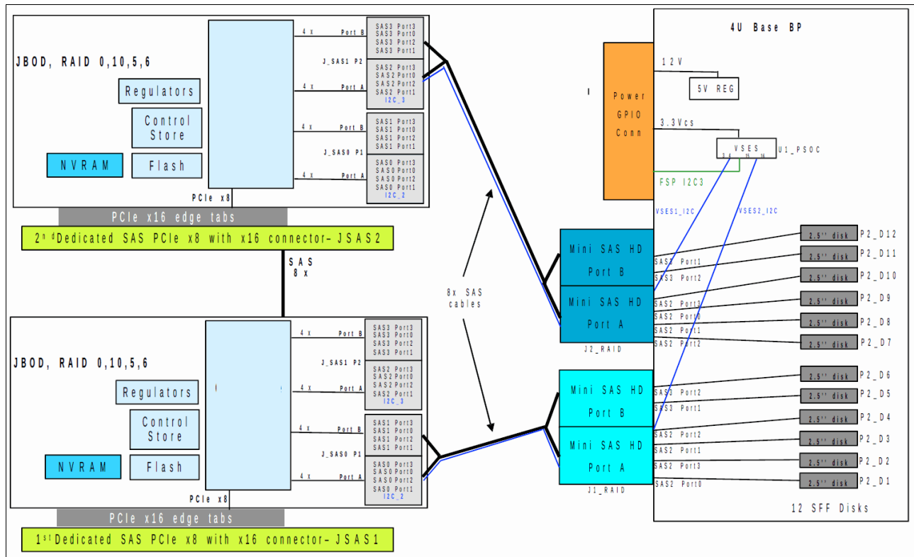
Figure 2-16 #EJ1E connections
