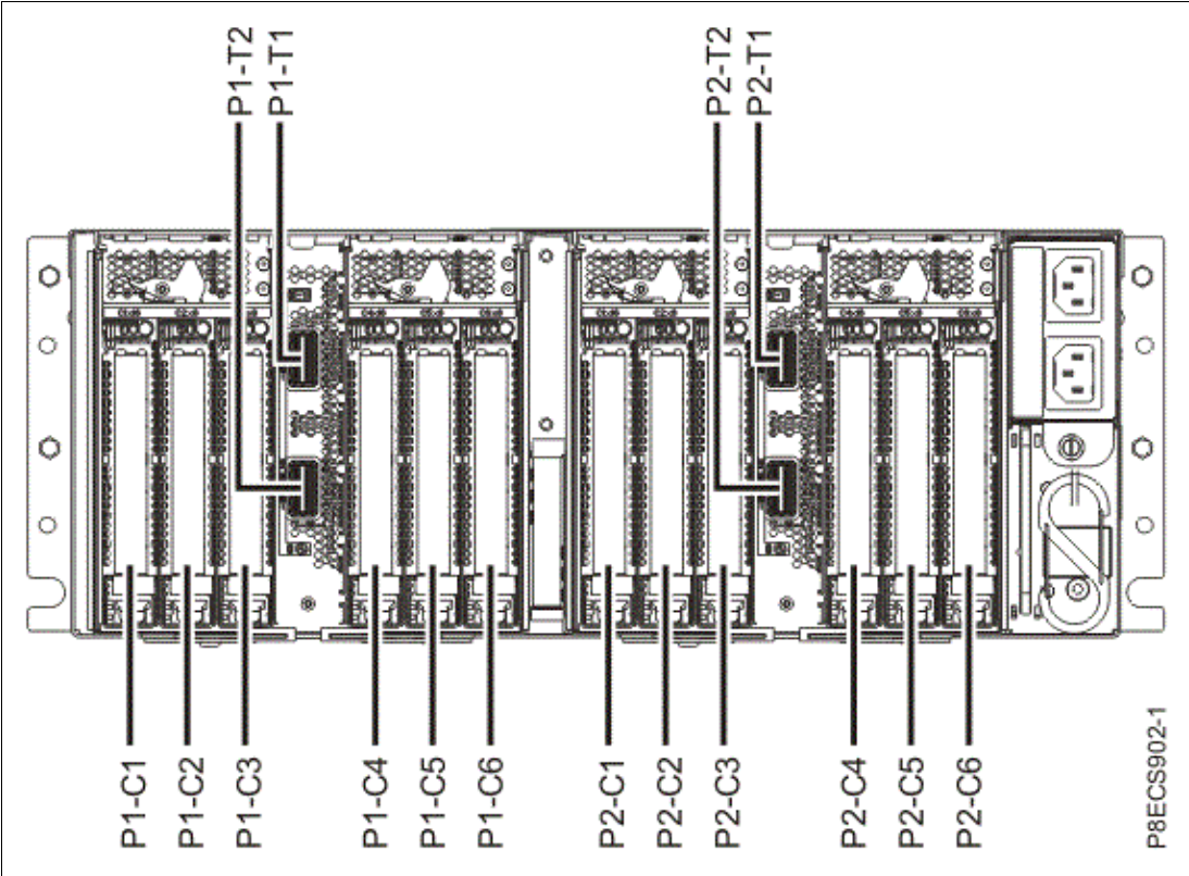
Figure 2-22 Connector locations for the PCIe Gen3 I/O expansion drawer
