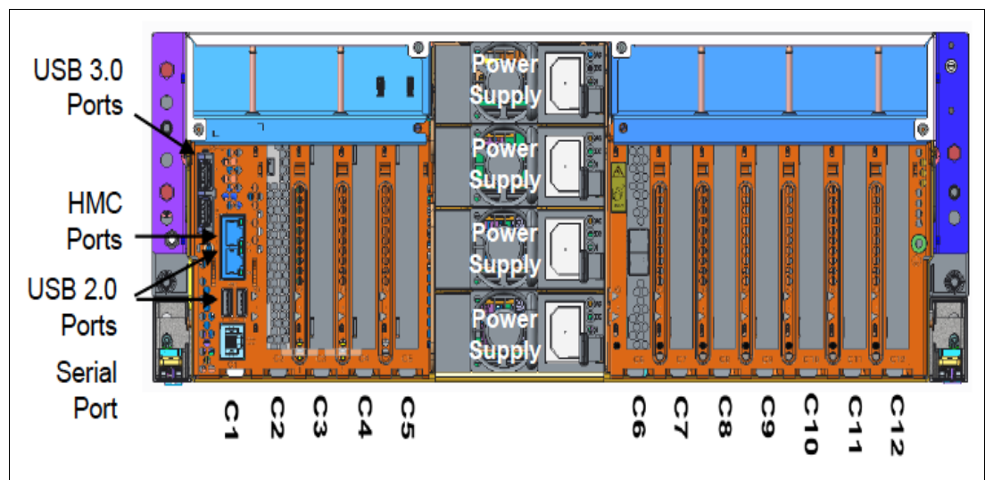
Figure 2-11 Rear view of a rack-mounted Power H924 system with PCIe slots location codes
