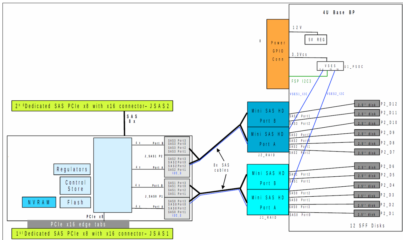
Figure 2-15 #EJ1C connections
