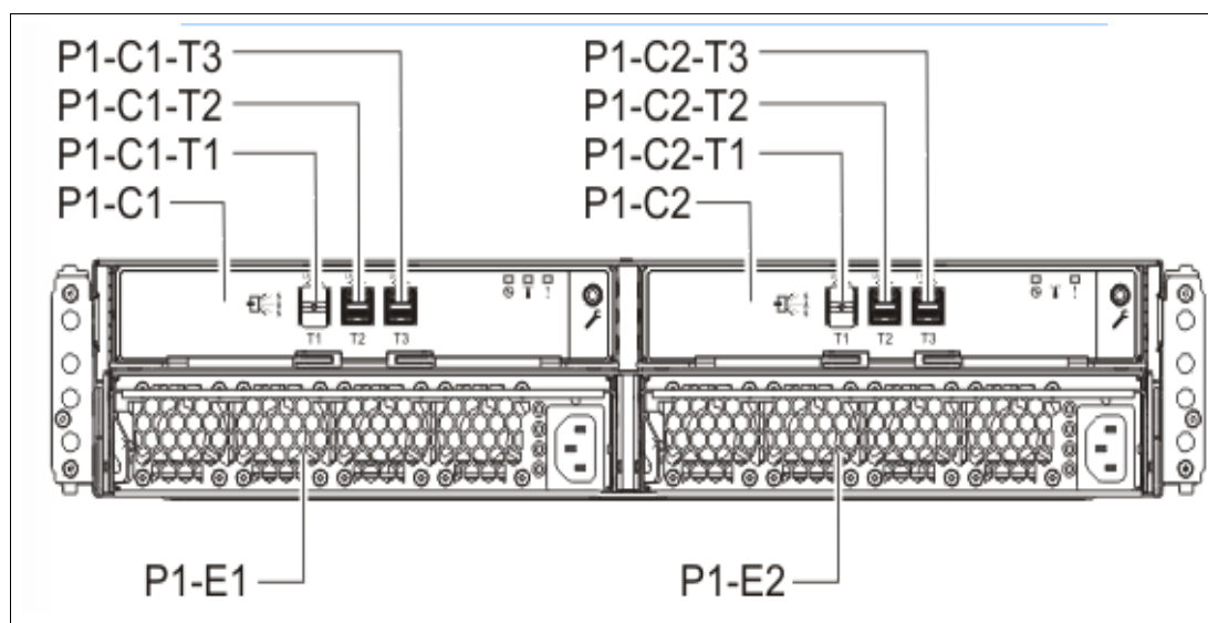
Figure 2-24 Connector locations for the EXP24SX and EXP12SX storage enclosures
