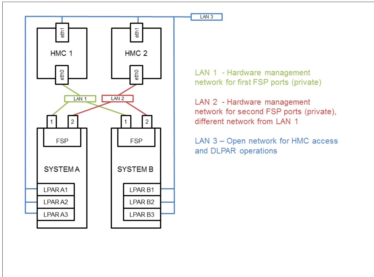
Figure 1-18 Highly available HMC networking example.
