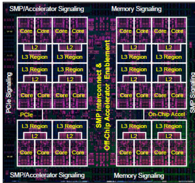
Figure 2-3 The 24-core POWER9 processor
