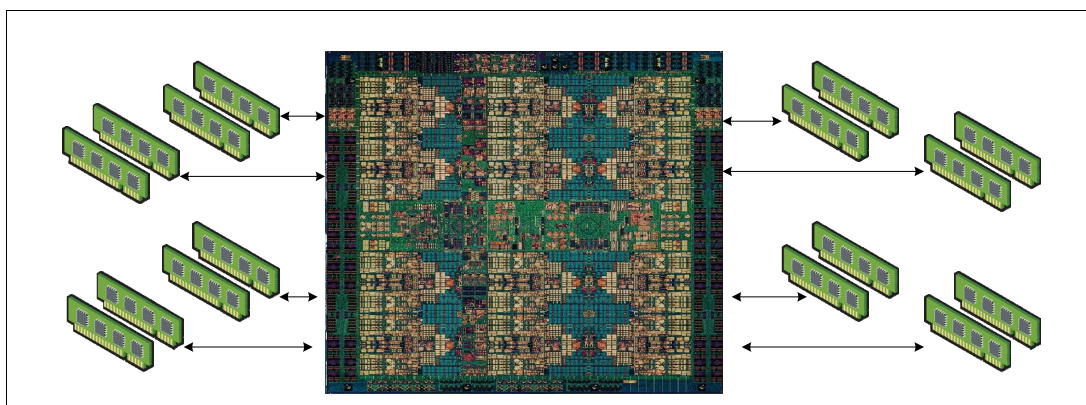
Figure 2-5 Overview of POWER9 direct-attached memory
