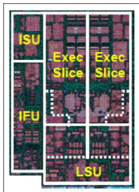
Figure 2-4 POWER9 SMT4 processor core
