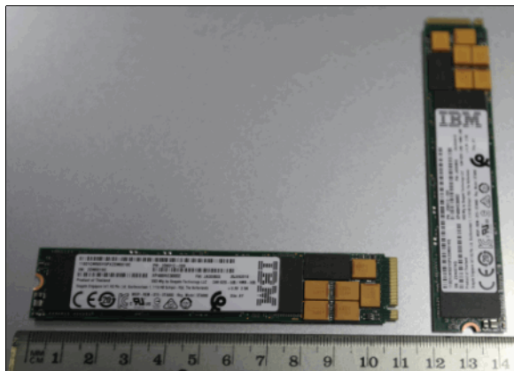
Figure 2-14 Two #ES14 NVMe modules
