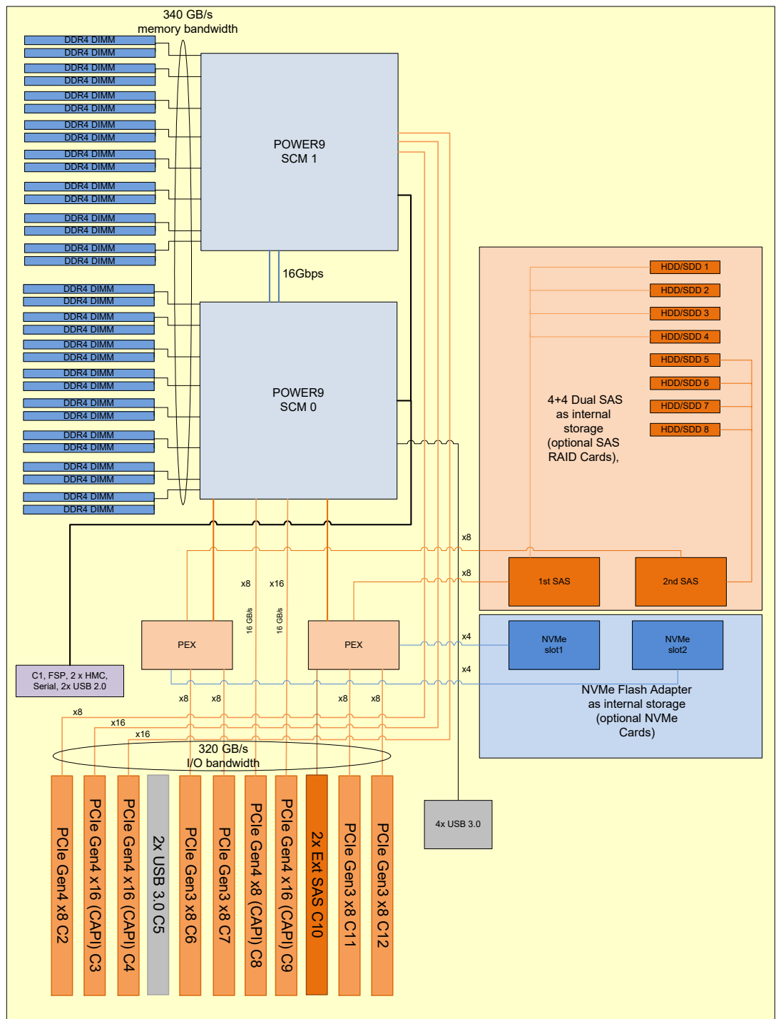
Figure 2-2 The IBM Power H922 logical system diagram
