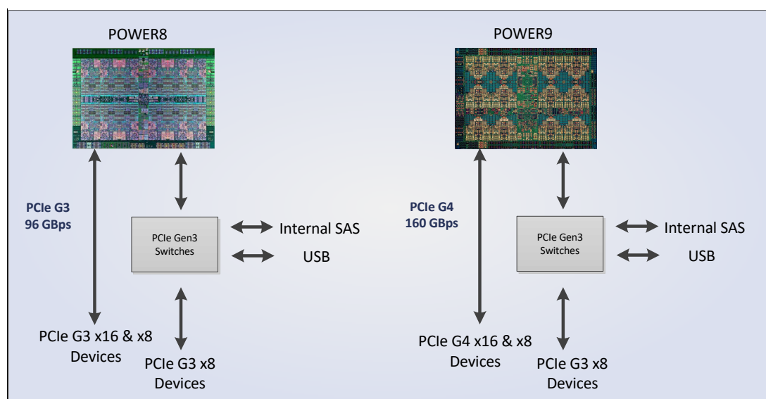
Figure 2-9 Comparison of POWER and POWER9 I/O buses architectures
