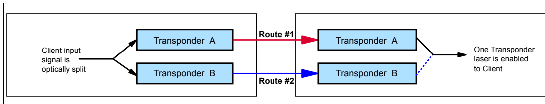
Figure 8 Y-Cable Line card protected scheme
