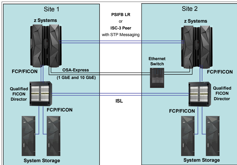
Figure 2 Multisite STP-only CTN
