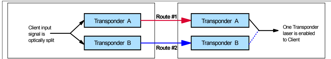
Figure 8 Y-Cable Line card protected scheme
