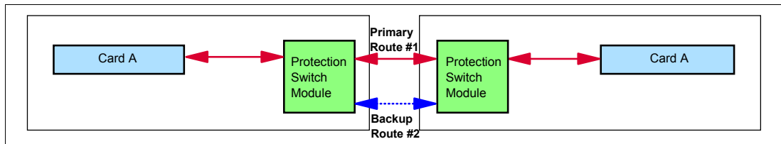
Figure 6 Optically Switched Fiber protection
