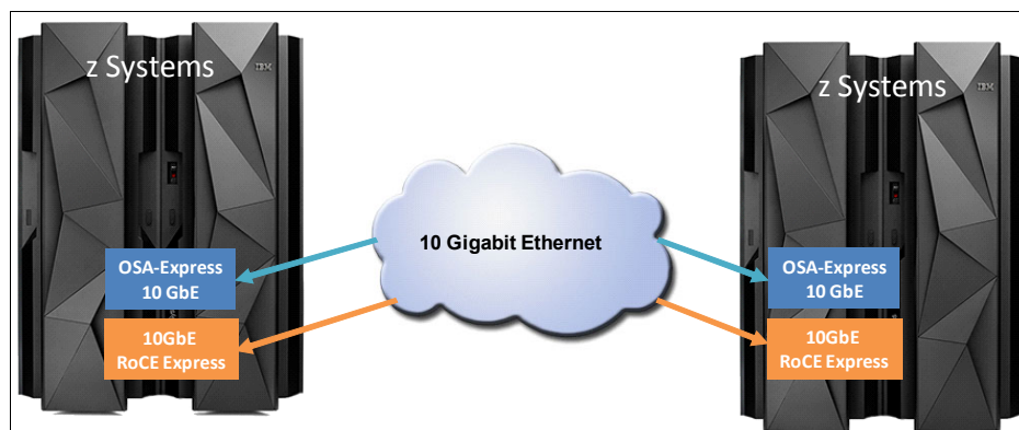
Figure 4 RoCE in a two site configuration through DWDM
