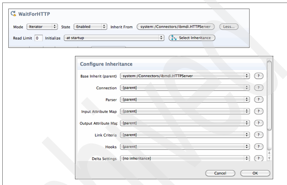
Figure 12 Configure inheritance
