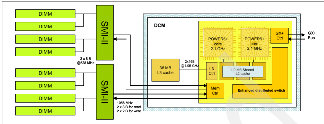
Figure 2-5 The p5-550 POWER5+ 2.1 GHz DCM with DDR2 memory socket layout view
