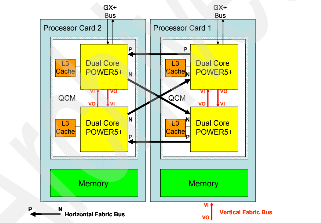
Figure 2-4 IBM System p5 550Q 8-core configuration
