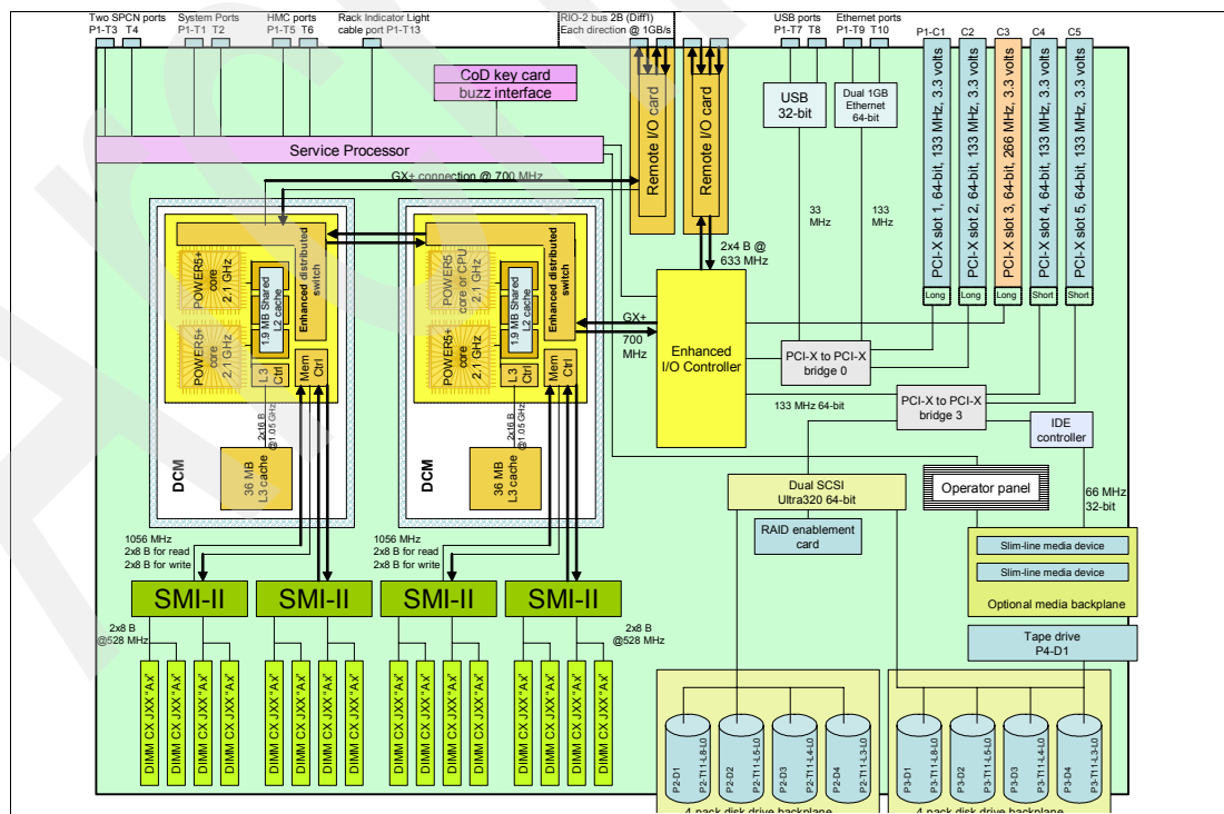
Figure 2-1 The IBM System p5 550 architecture with 2.1 GHz DCM
