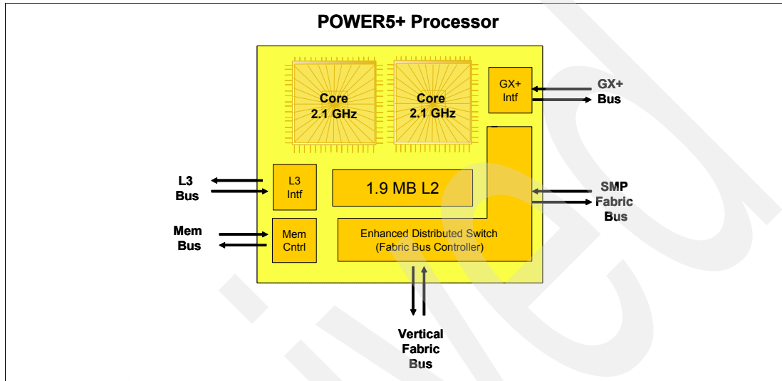
Figure 2-2 POWER5+ processor
