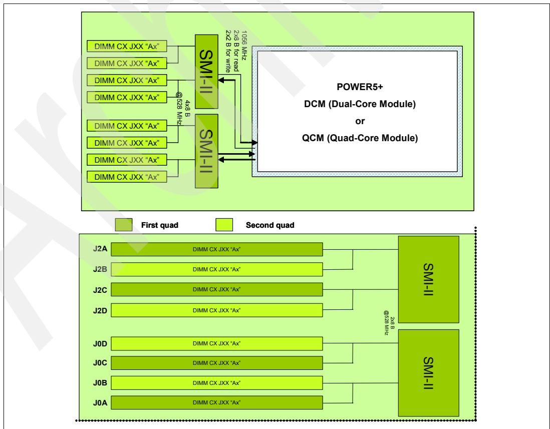
Figure 2-6 Memory placement for the DCM or QCM
