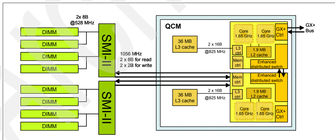
Figure 2-3 p5-550Q POWER5+ 1.65 GHz QCM processor card with DDR2 memory socket layout view
