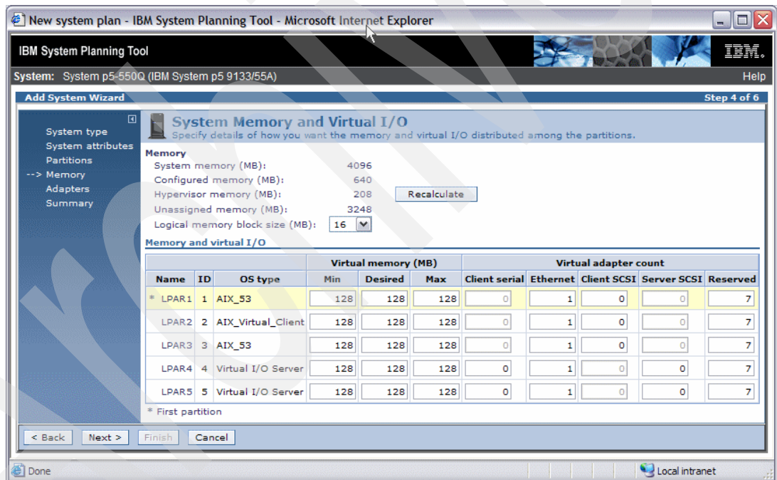
Figure 2-18 IBM System Planning Tool window showing Hypervisor requirements
