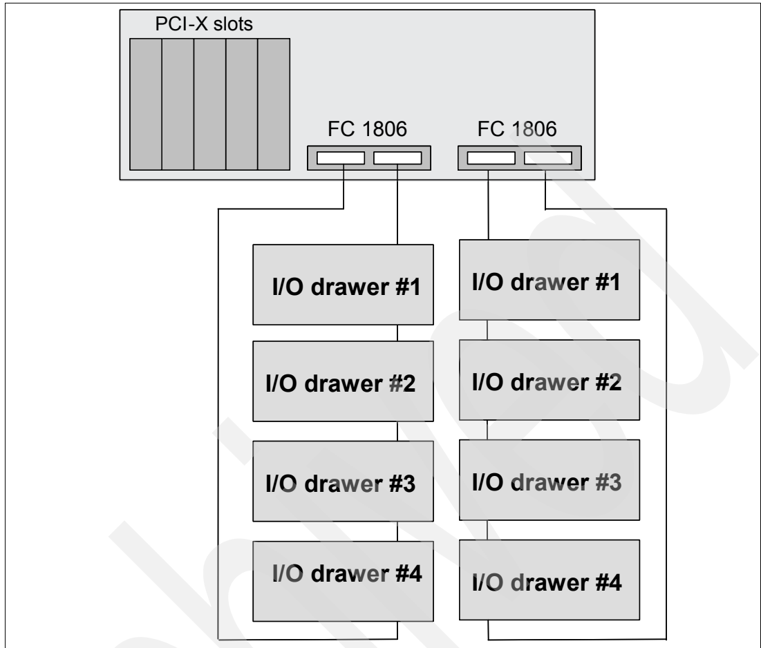
Figure 2-11 RIO-2 connections
