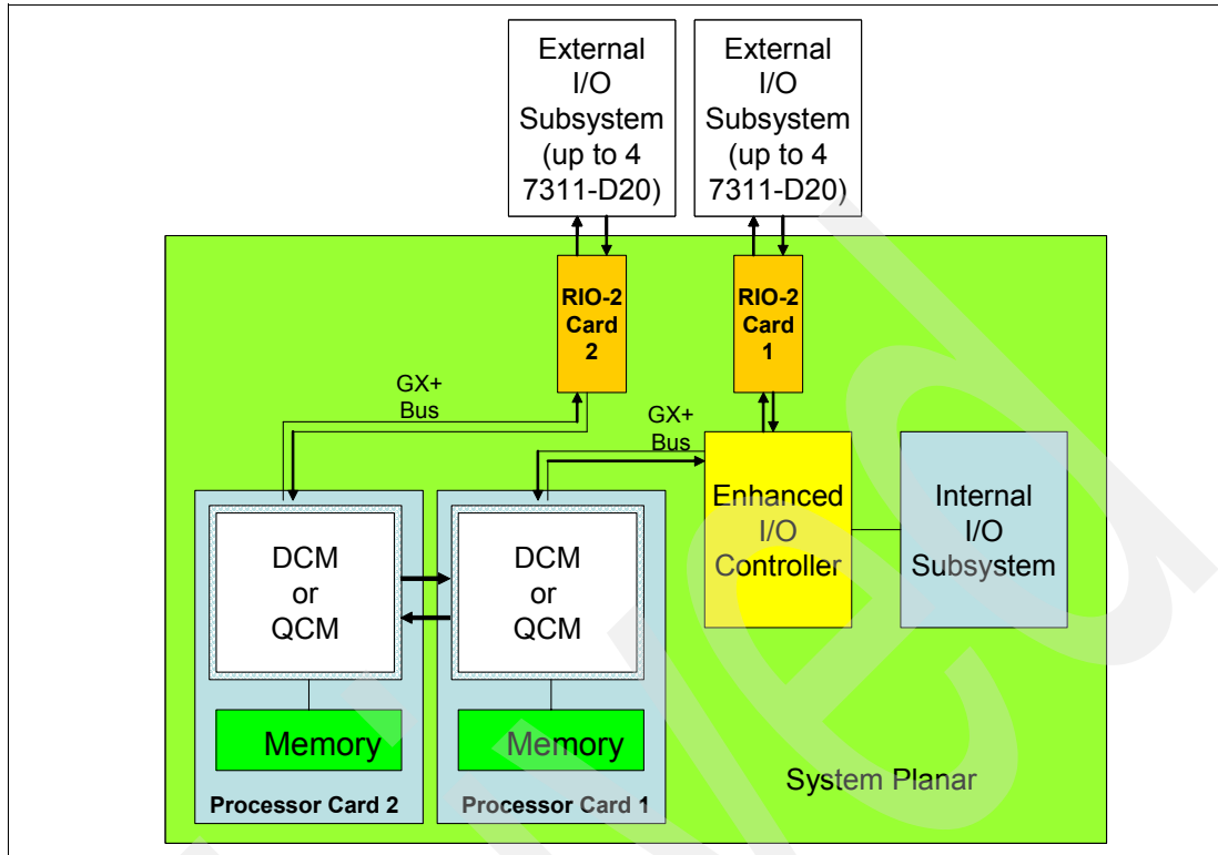
Figure 2-8 The p5-550 or p5-550Q GX+ Bus connections overview
