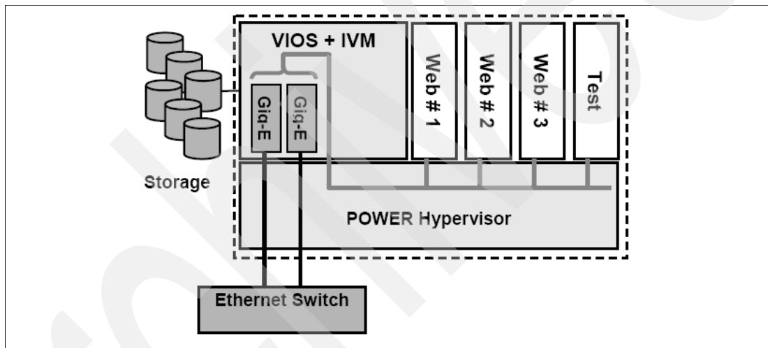
Figure 2-15 IVM principles
