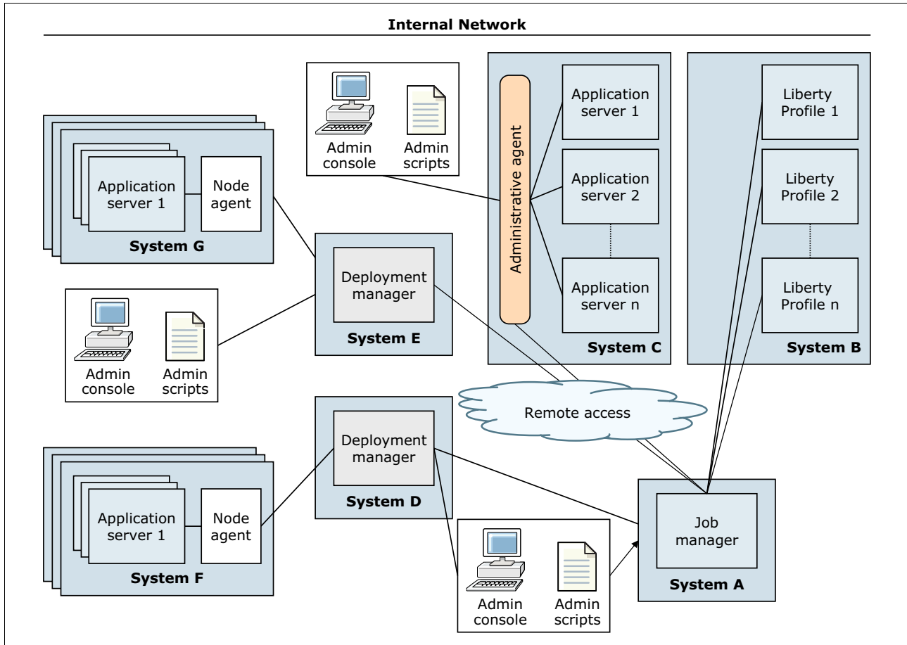
Figure 8-15 Topology using a job manager
