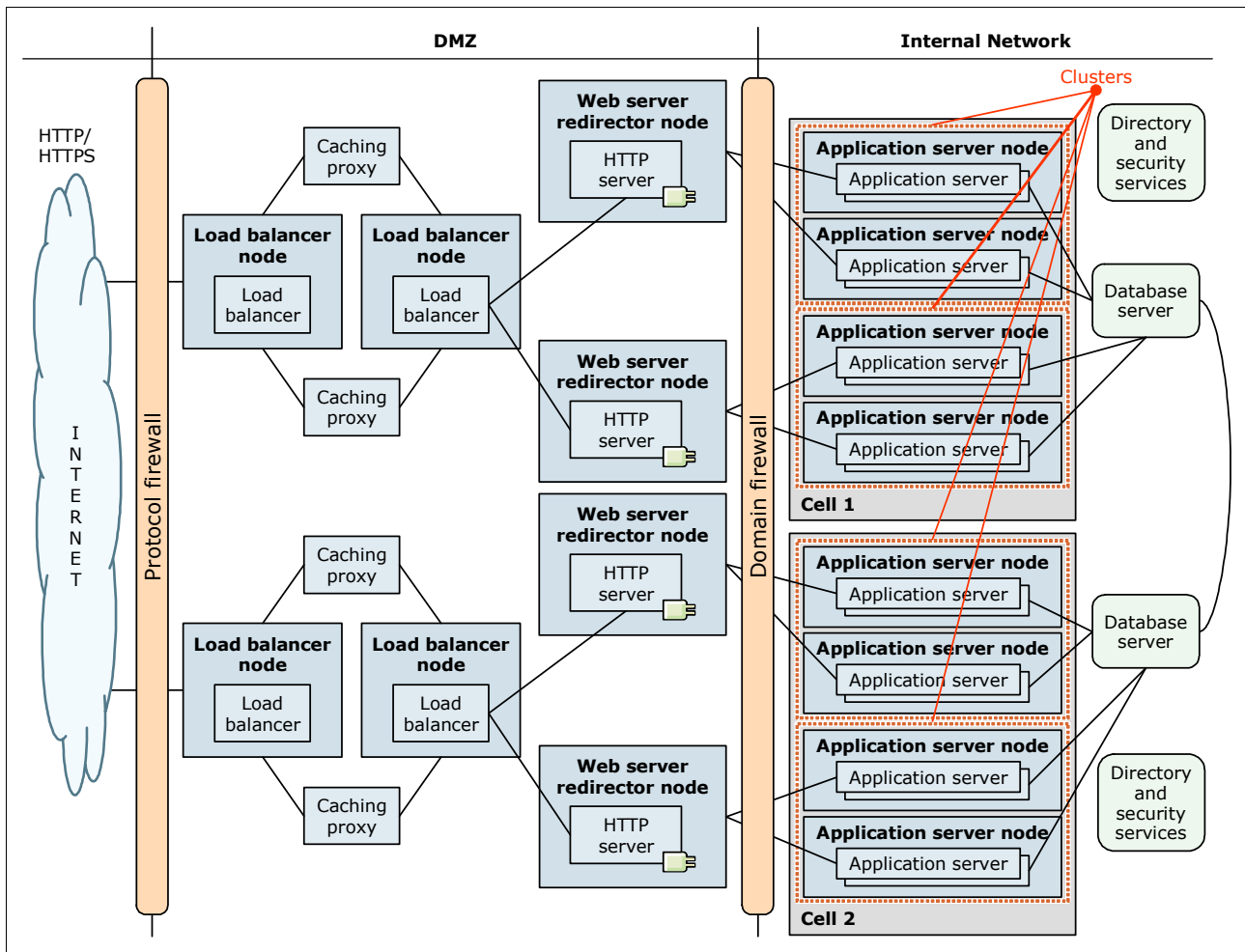
Figure 8-12 Multi-cell architecture
