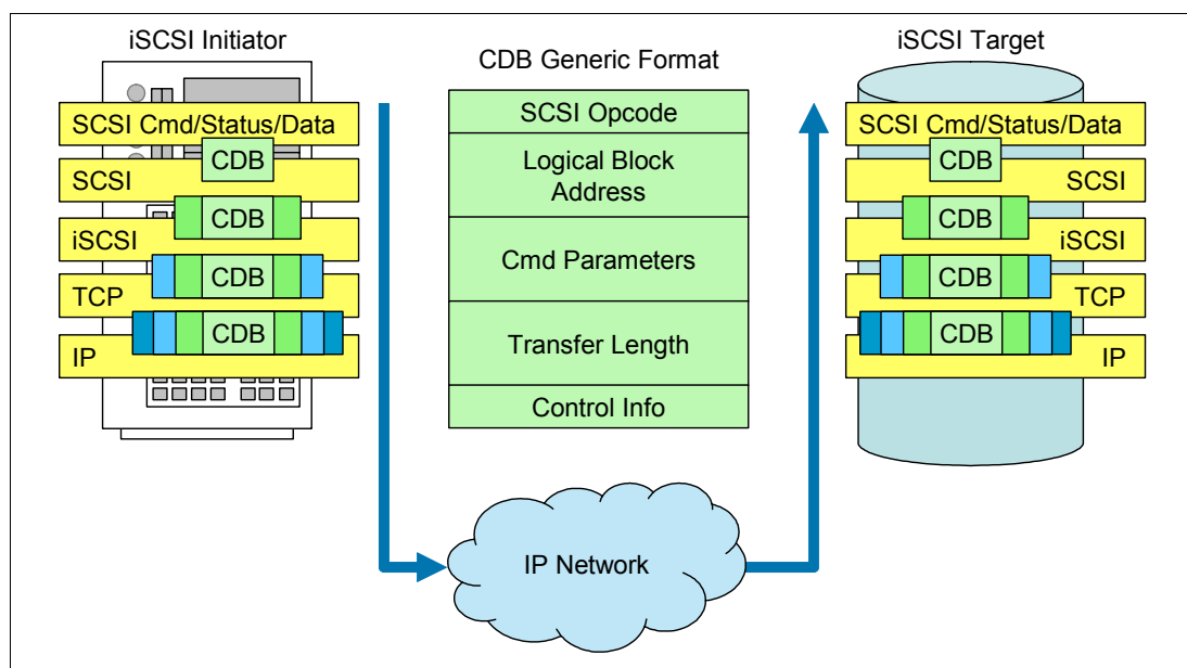
Figure 3-2 iSCSI protocol layers
