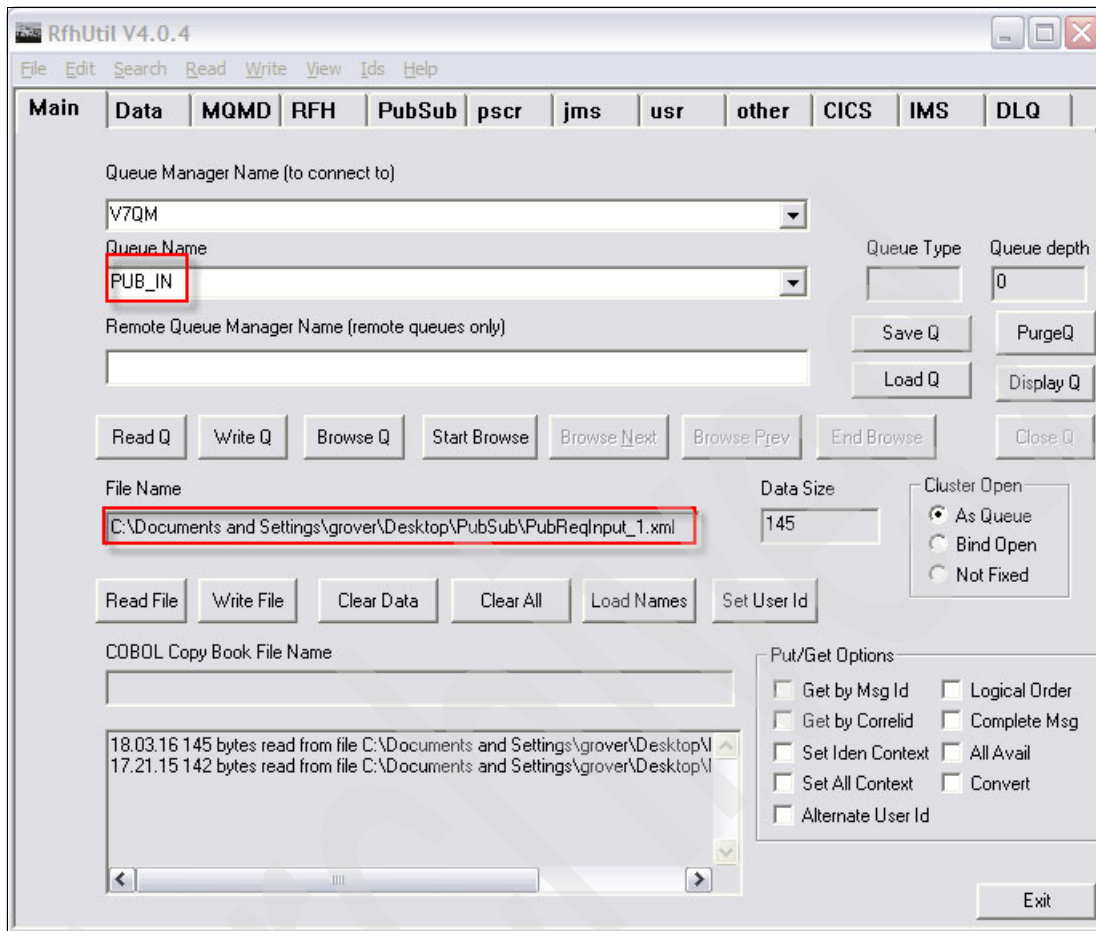
Figure 9-70 Send publication to the Publisher message flow
