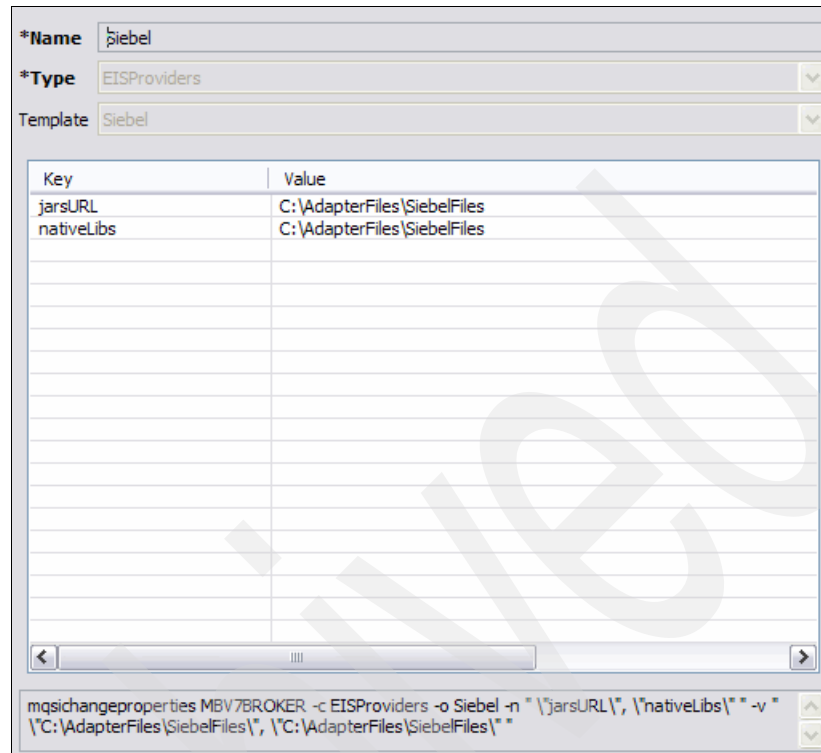
Figure 6-51 The mqsichangeproperties command
