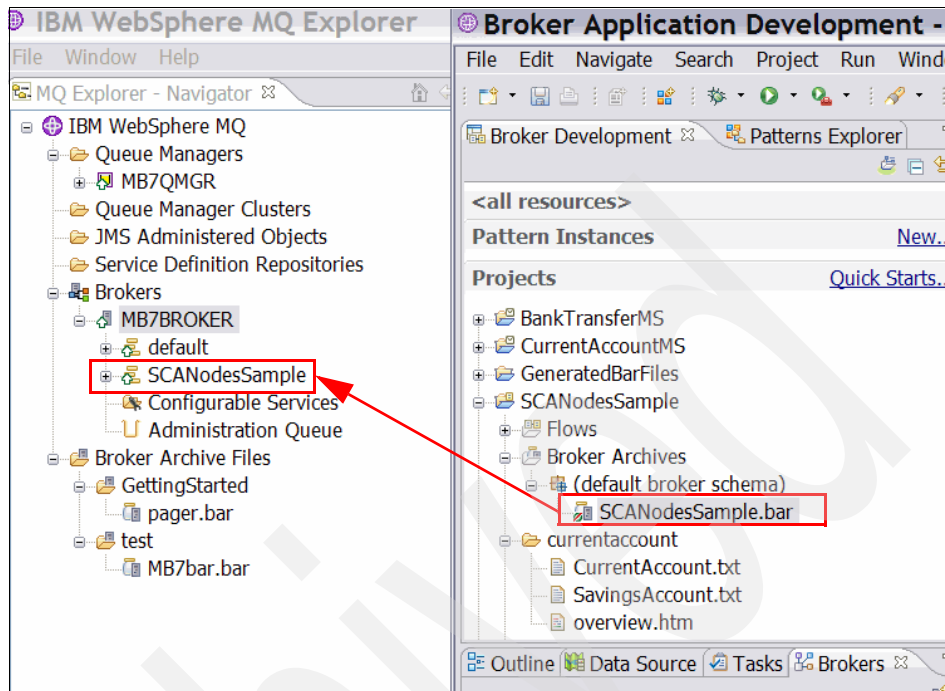
Figure 5-38 Drag SCANodesSample bar file from development toolkit onto the EG on MQ Explorer
