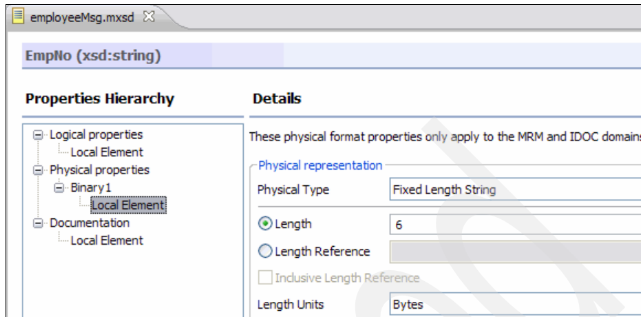
Figure 8-27 Local element EmpNo properties
