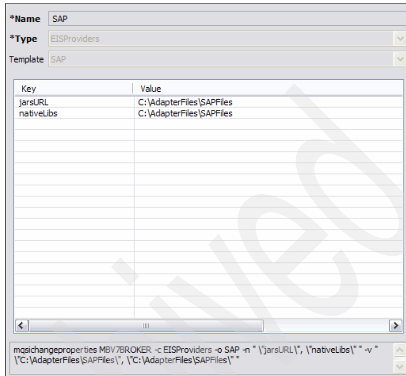
Figure 6-50 The mqsischangeproperties command
