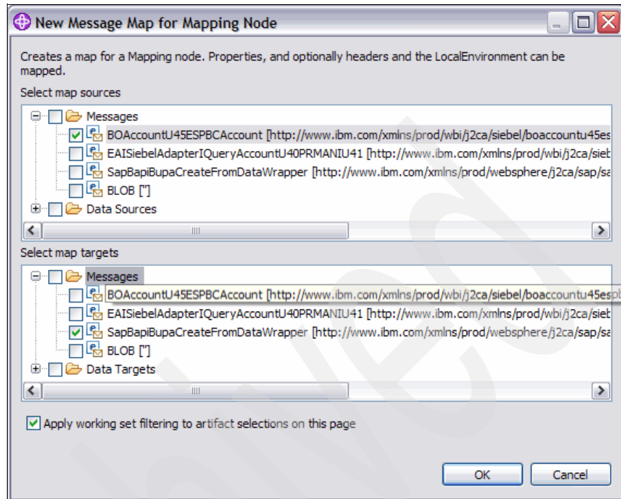
Figure 6-81 Mapping between the Siebel and SAP formats
