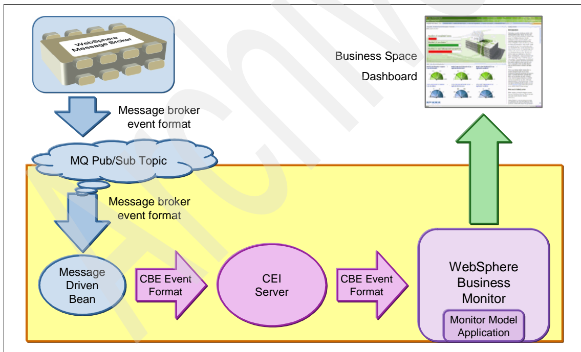
Figure 10-1 System architecture
