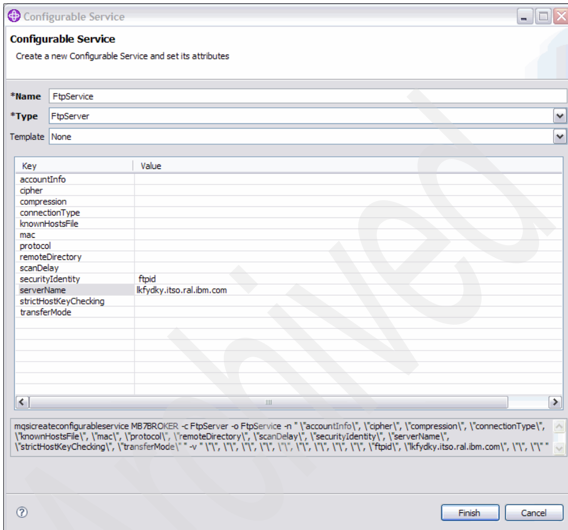
Figure 8-22 Configurable Service window
