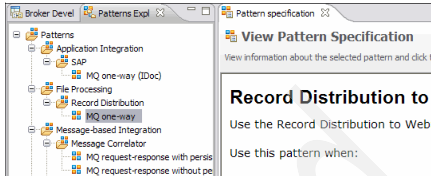
Figure 8-28 Pattern Explorer
