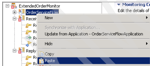
Figure 10-81 ReceiveExit paste
