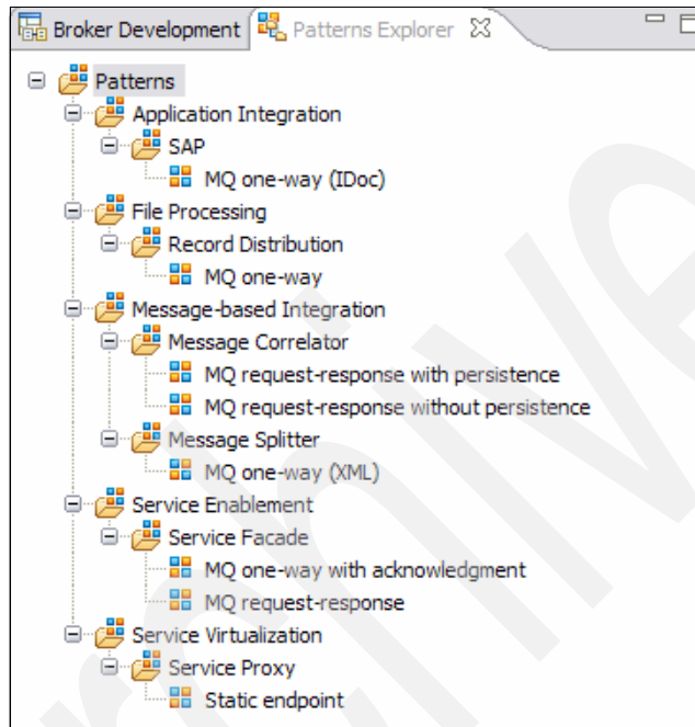
Figure 2-3 Patterns Explorer
