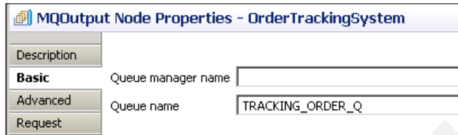
Figure 10-32 MQOutput properties
