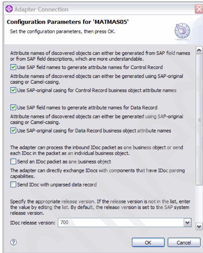
Figure 6-9 Adapter Connection wizard: Configure MATMAS05
