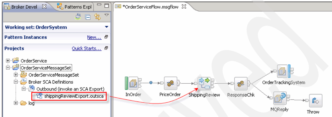
Figure 10-30 Importing the SCAResponse node
