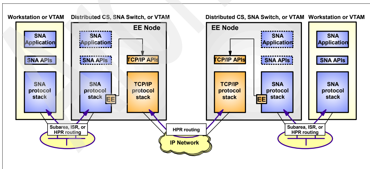
Figure 3-16 Enterprise Extender sample topology
