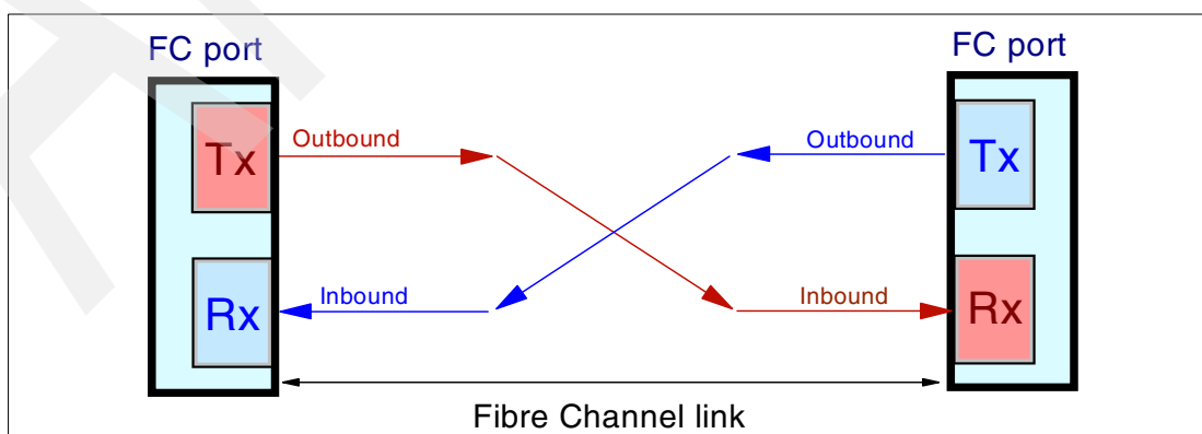
Figure 2-2 Fibre Channel link
