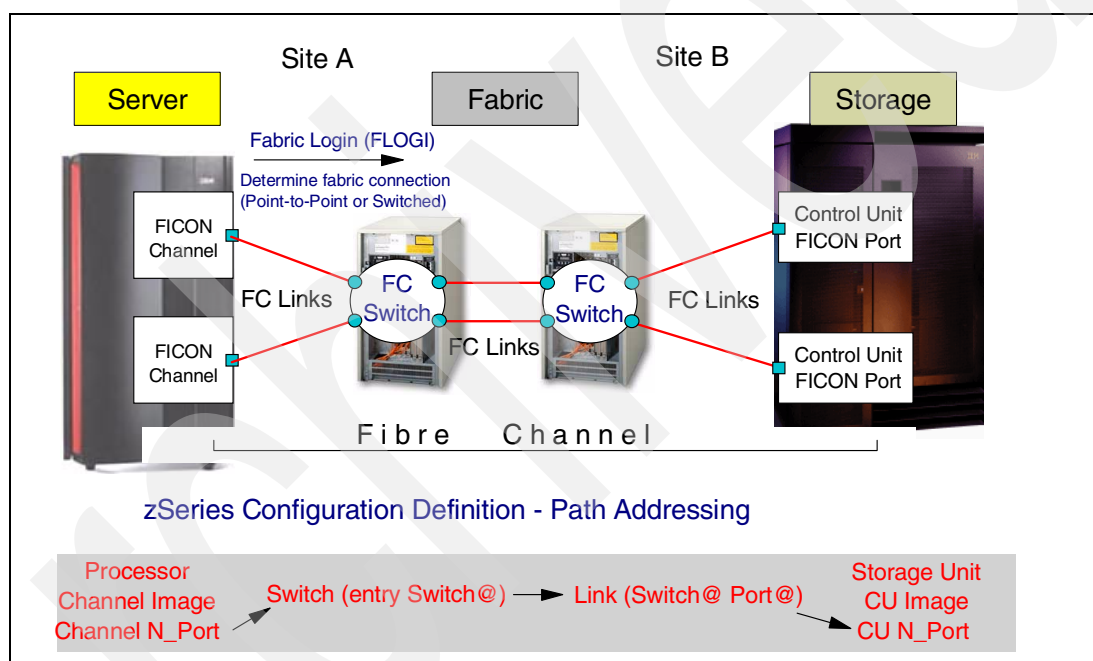
Figure 2-7 FICON native Cascaded FICON Directors configuration
