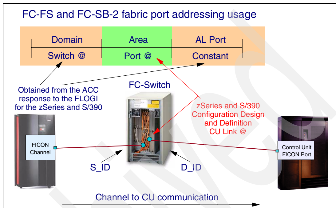
Figure 3-12 FICON single switch - switched point-to-point link address
