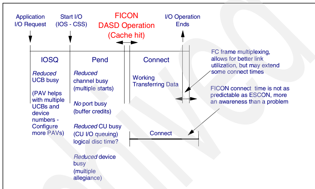
Figure 11-13 FICON I/O operation sequence - cache hit
