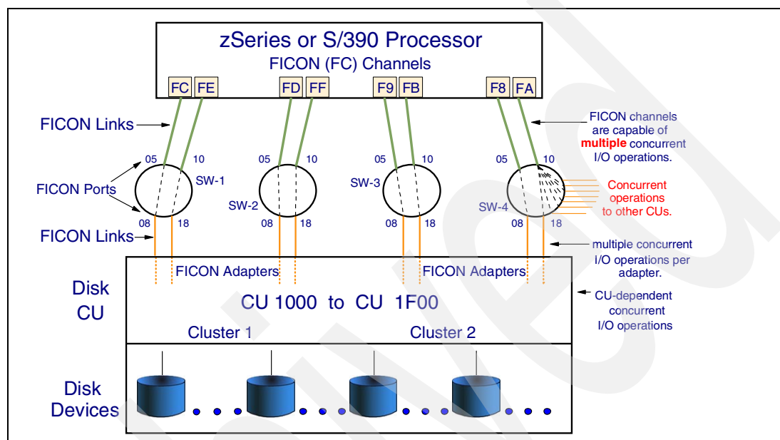
Figure 7-8 FICON switched point-to-point channel configuration with eight paths
