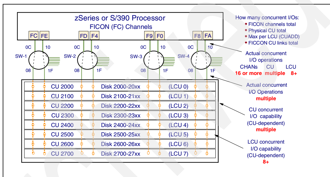
Figure 7-14 FICON channel configuration - 8 channel paths to 8 LCUs
