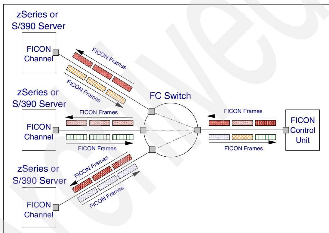
Figure 3-25 FICON frame transfer in a multi-system environment
