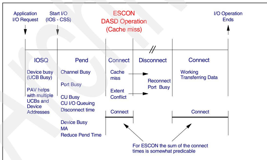
Figure 11-12 ESCON I/O operation sequence - cache miss
