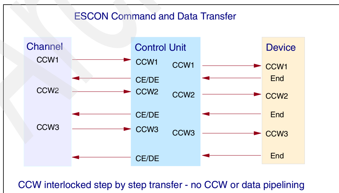
Figure 11-3 ESCON command and data transfer
