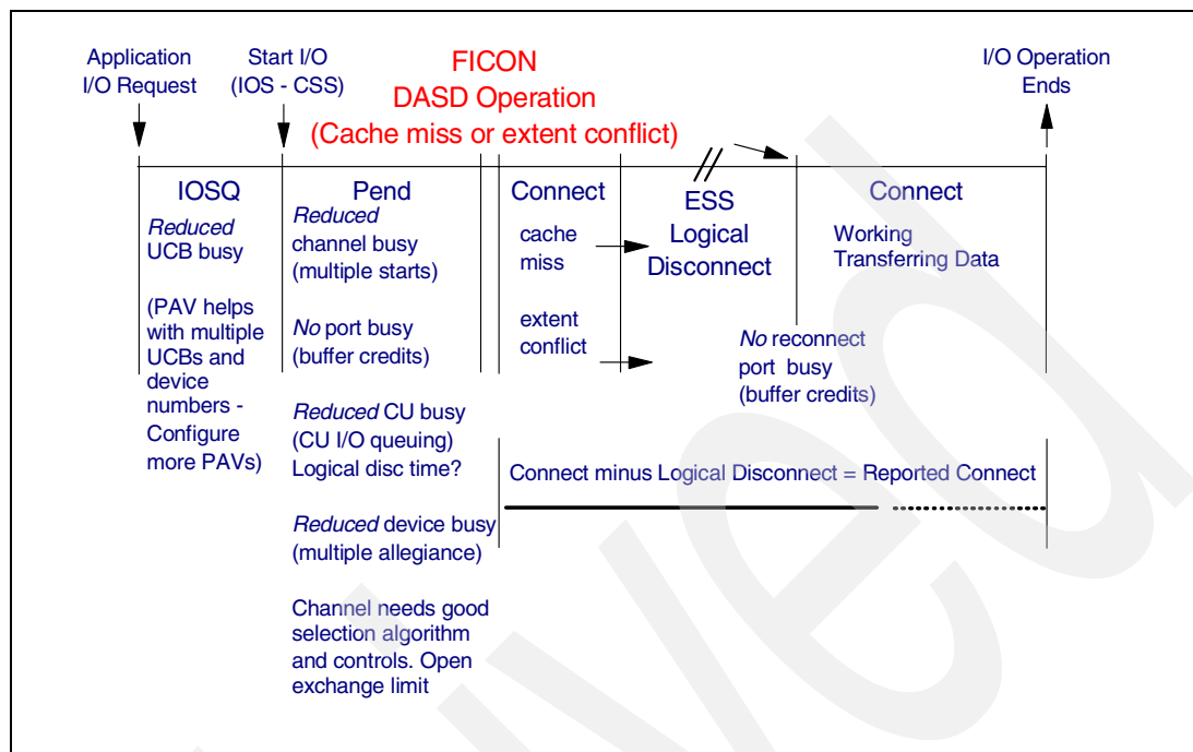
Figure 11-14 FICON I/O operation sequence - cache miss
