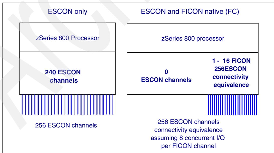
Figure 4-5 zSeries 800 ESCON and FICON channel connectivity equivalence
