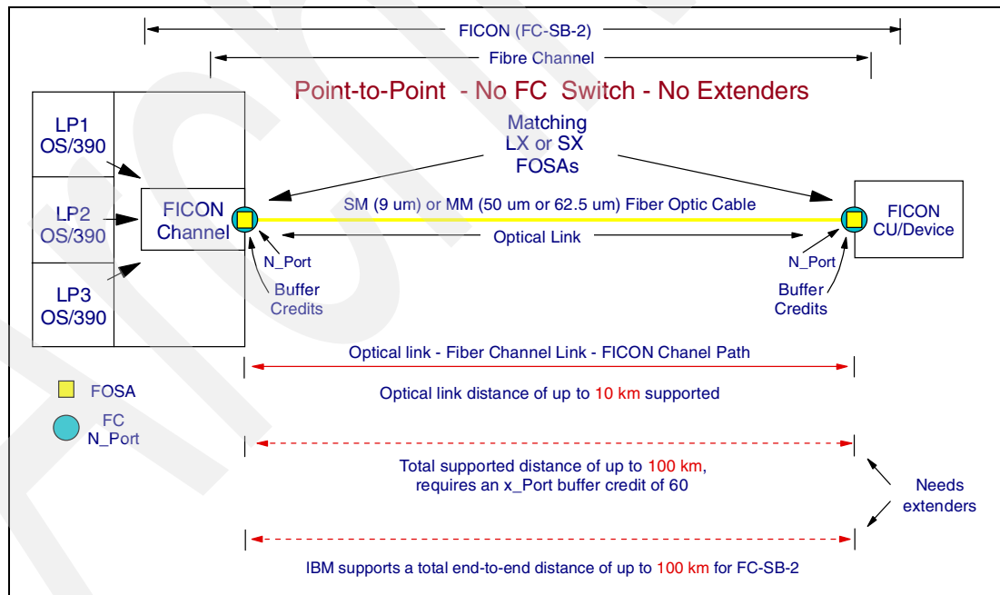
Figure 5-5 Point-to-point distances
