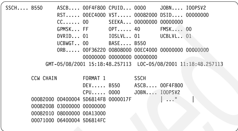
Figure F-12 GTF trace example (I/O request)
