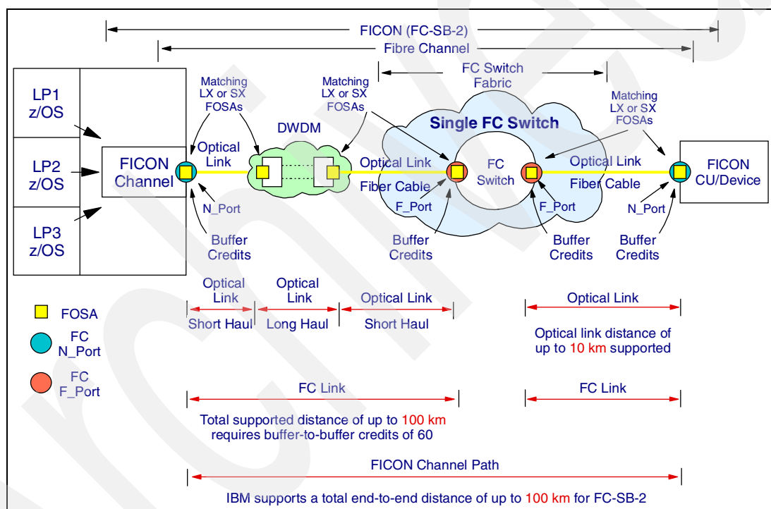
Figure 5-7 Switched point-to-point distances, using DWDM
