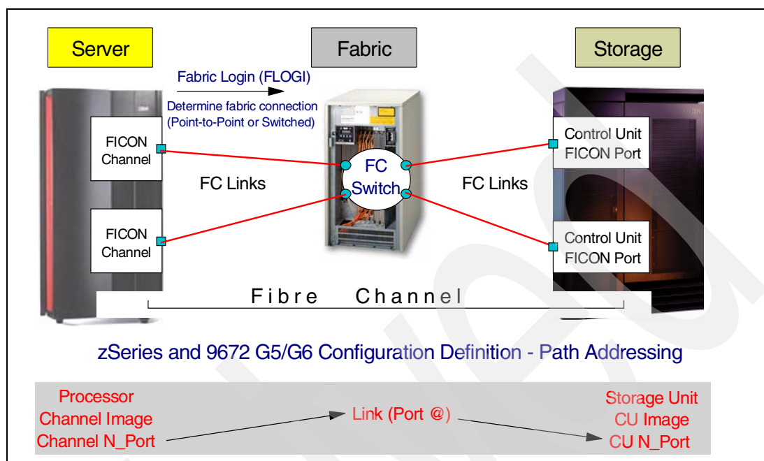
Figure 2-6 FICON native switched point-to-point configuration
