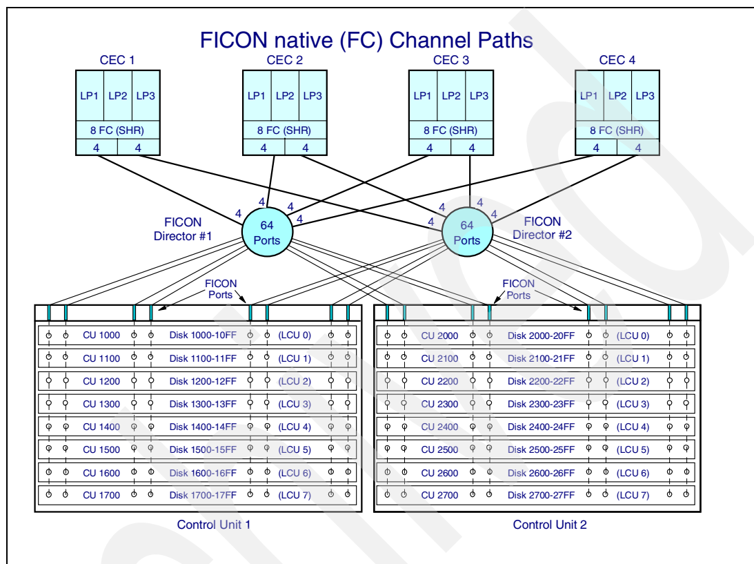
Figure 9-4 Migration scenario #1 - sample FICON native (FC) configuration
