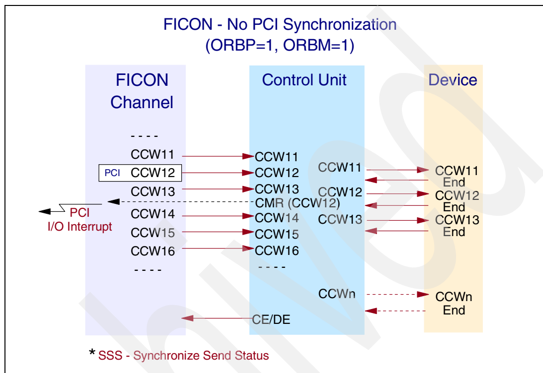
Figure 11-8 No PCI synchronization
