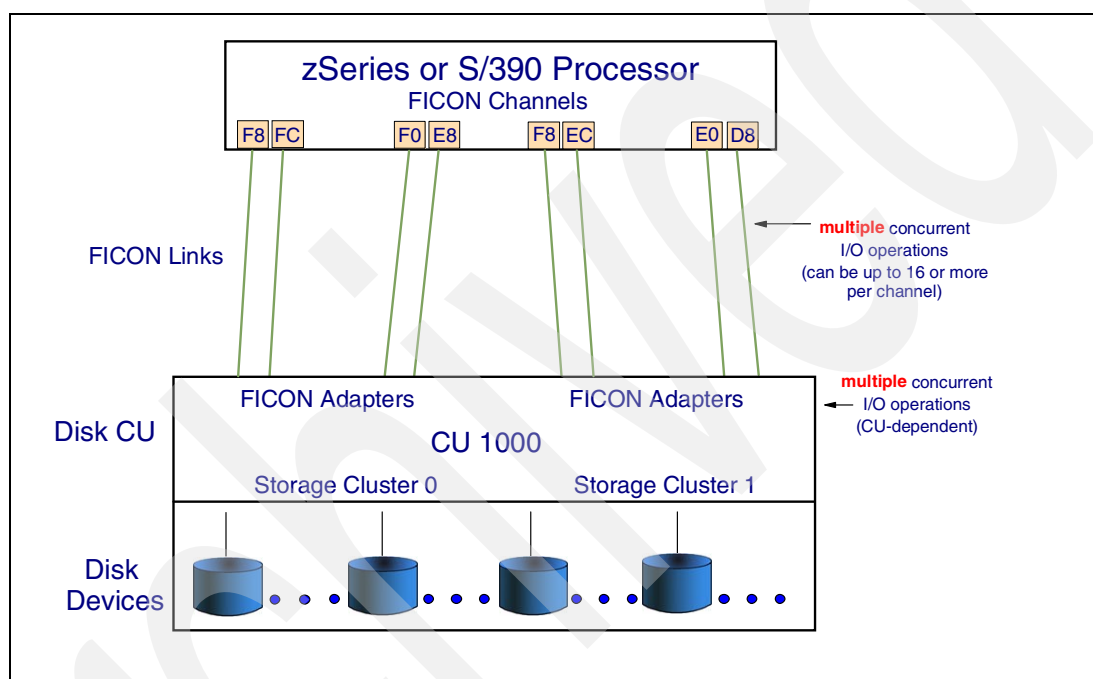
Figure 7-2 FICON point-to-point configuration
