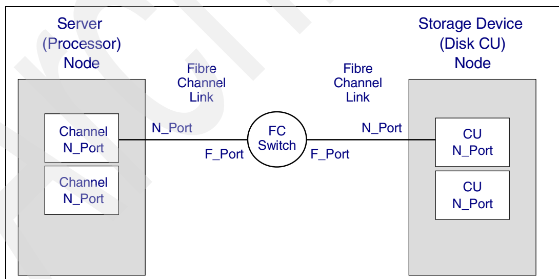
Figure 3-3 FICON switched point-to-point N_Port to N_Port communication
