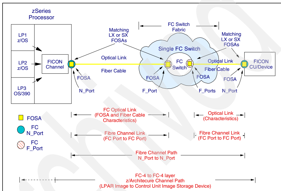
Figure 5-2 Basic FICON cabling terminology
