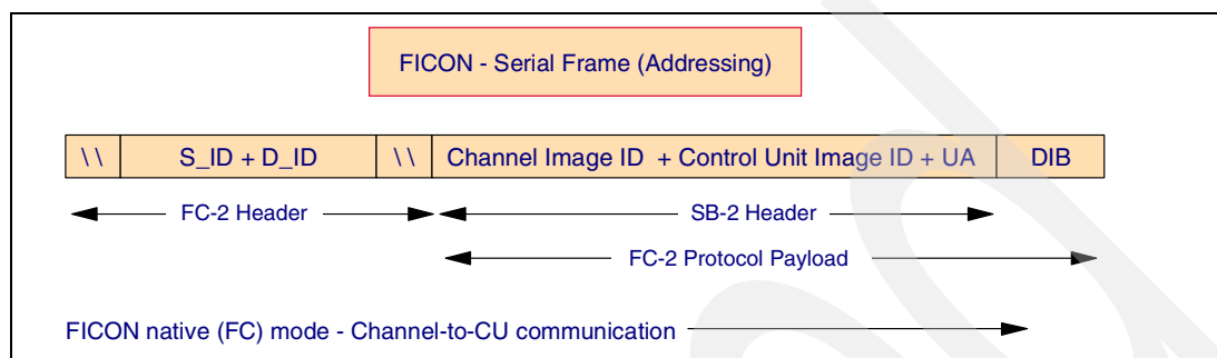
Figure 3-16 FICON native (FC) mode N_Port and device addressing
