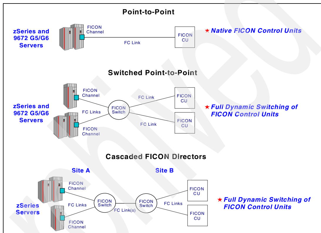
Figure 2-4 FICON connections and topologies
