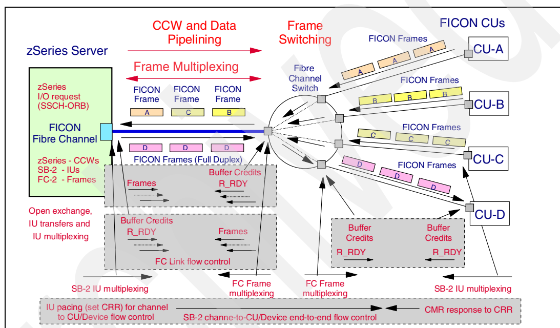
Figure 3-30 Fibre Channel buffer credits
