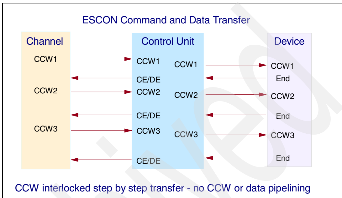
Figure 3-28 CCW operation on an ESCON channel
