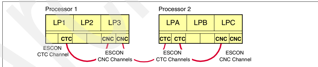
Figure 10-2 ESCON point-to-point CTC connection, multiple processors
