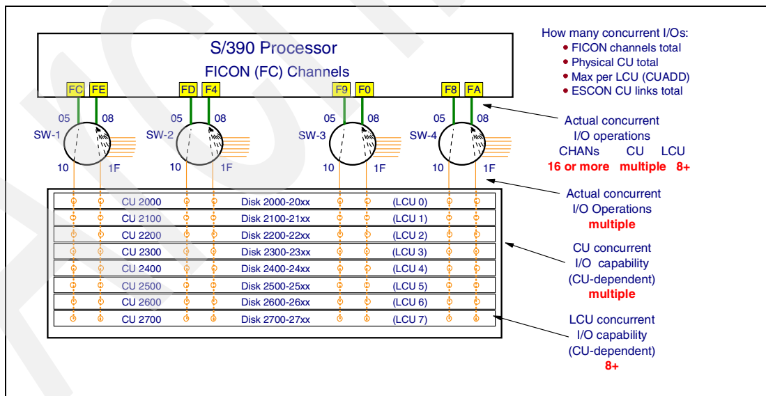
Figure 7-25 FICON channel configuration - 8 channels to 8 LCUs
