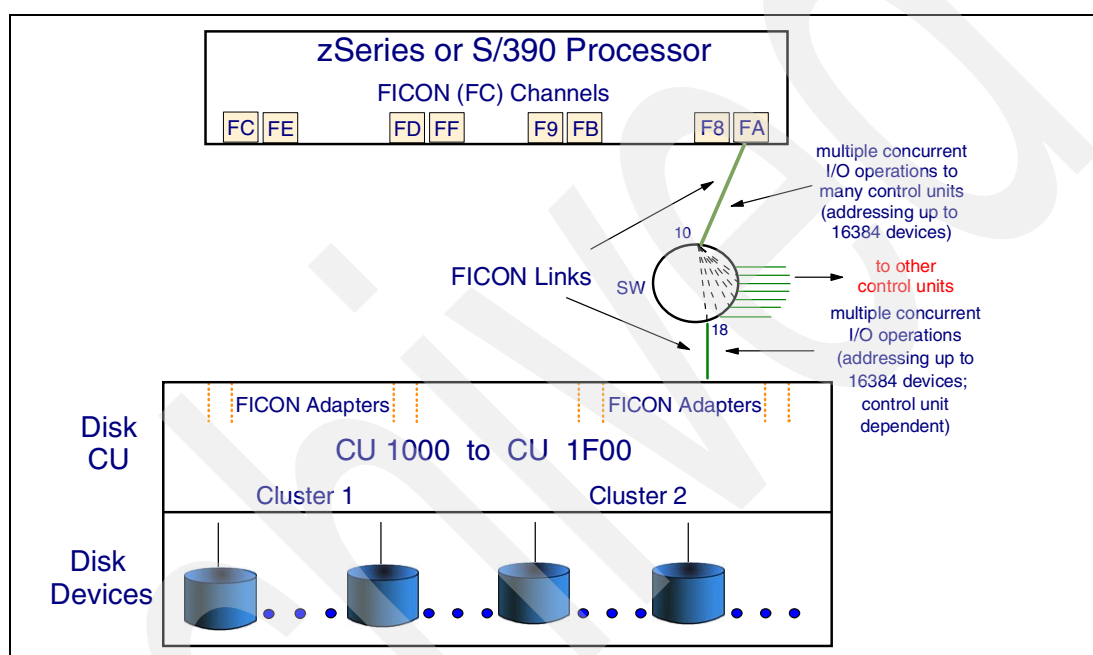
Figure 7-9 Single FICON channel I/O concurrency
