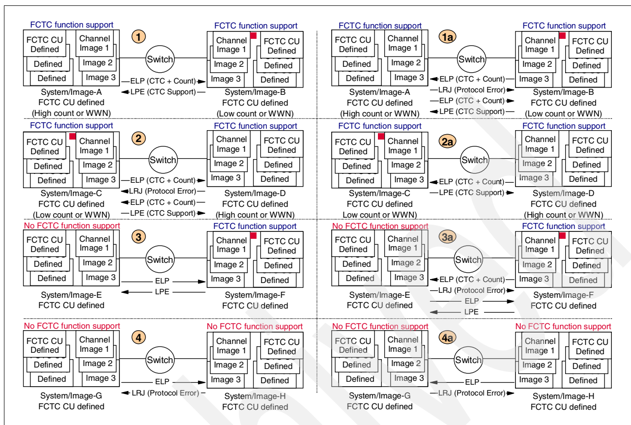
Figure 10-21 FICON CTC control unit establishment algorithm
