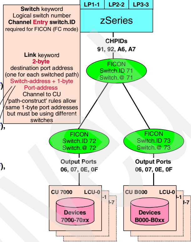
Figure E-2 Two switch cascaded configuration (two fabrics, one control unit each)
