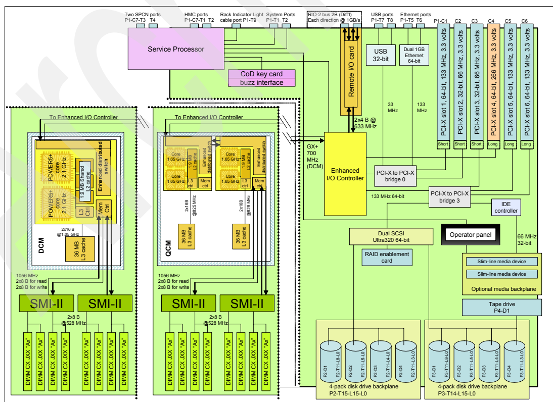
Figure 2-1 IBM System p5 520 and IBM System p5 520Q architecture with QCM or DCM
