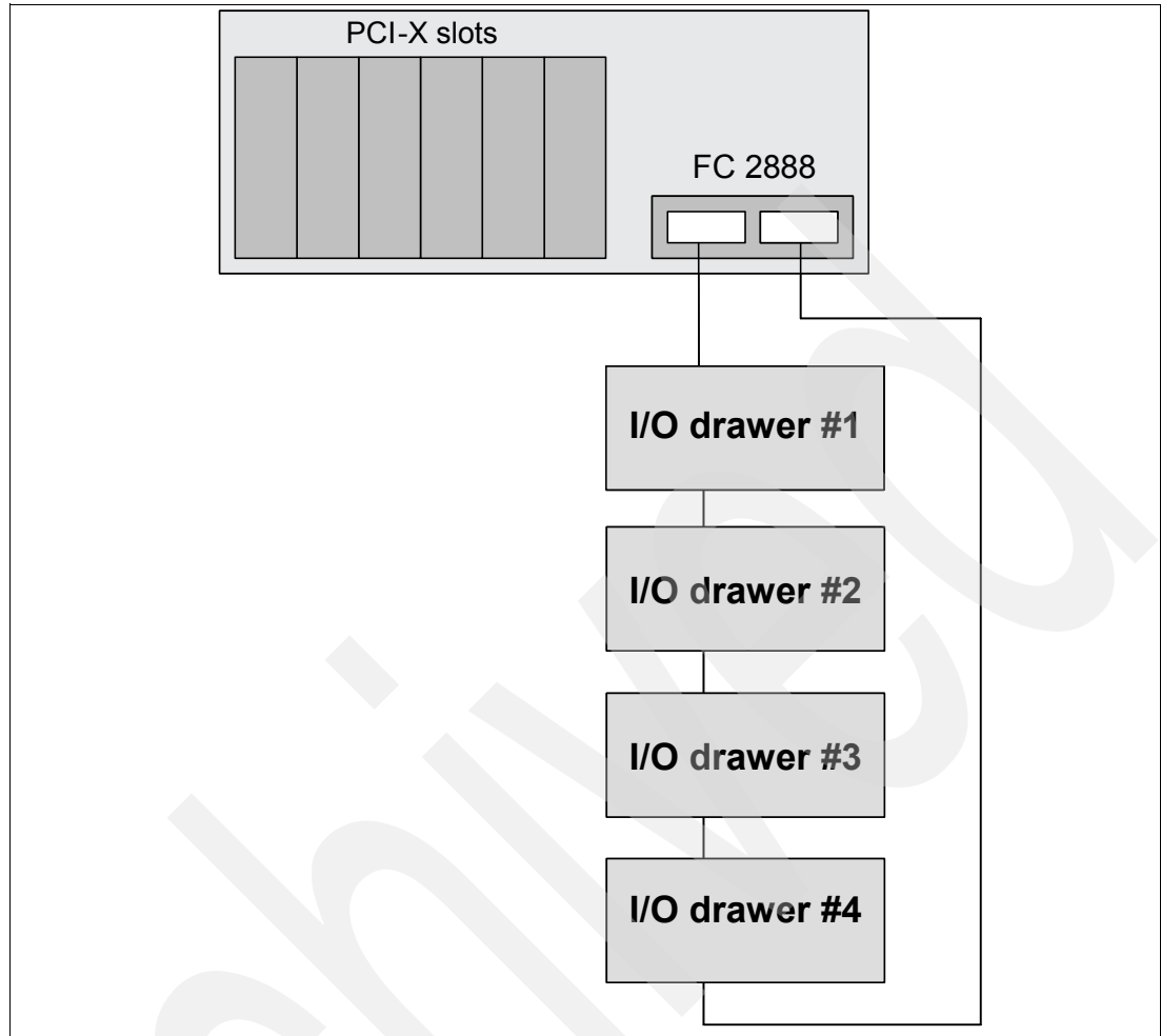
Figure 2-12 RIO-2 connections
