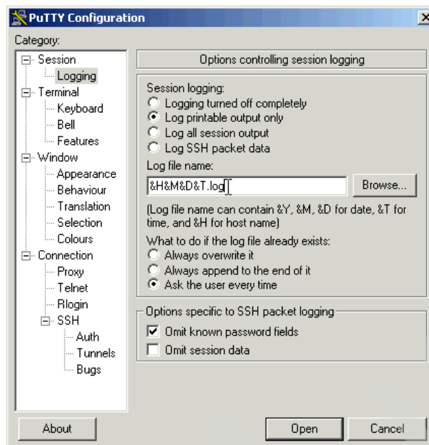
Figure 3-2 Setting Logging
