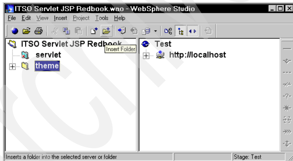
Figure 171. Studio Workbench
