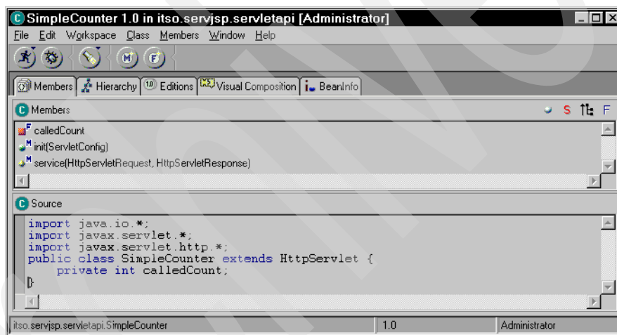
Figure 138. Class browser
