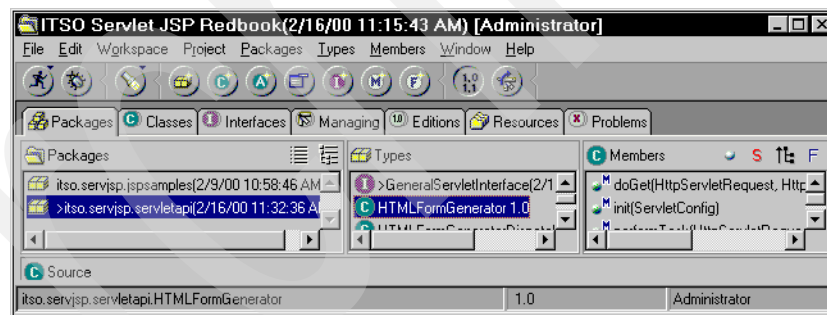
Figure 136. Project browser
