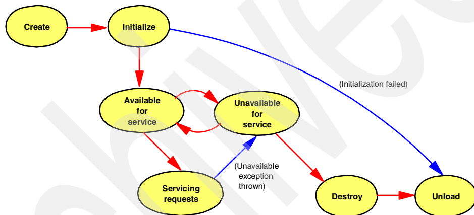
Figure 33. Servlet life-cycle
