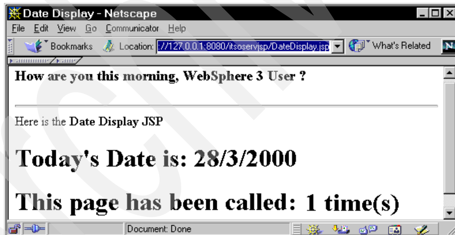
Figure 155. DateDisplay.jsp output
